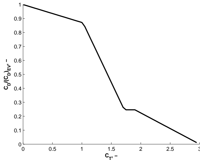
Figure 7. Drag coefficient variation with thrust coefficient for supersonic retropropulsion.
