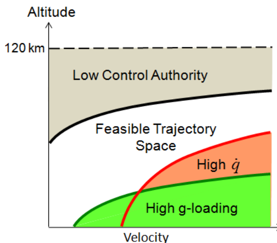
Figure 4. Entry corridor.
