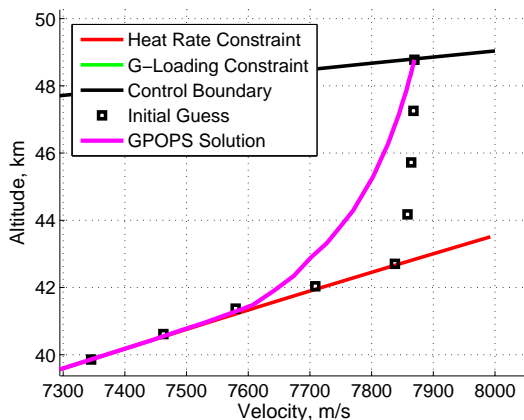
Figure 8. Beginning of converged pseudospectral solution.
