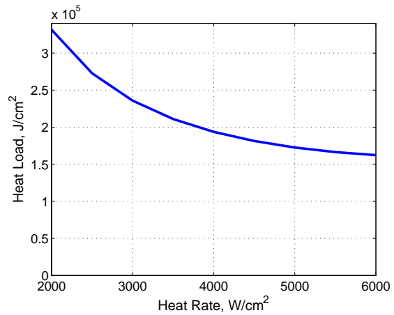
Figure 18. Optimal trade in heat rate constraint and minimum heat load.
