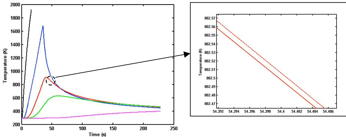
Figure 15. Non-nominal parameters result in the same thermal response as the nominal parameters
