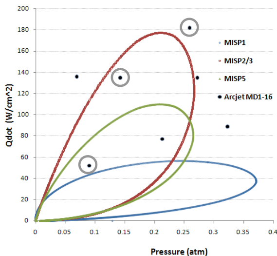
Figure 4. Predicted MISP heating environment and Arcjet test conditions (left), Post-test AHF 271 Iso-q sample (right)
