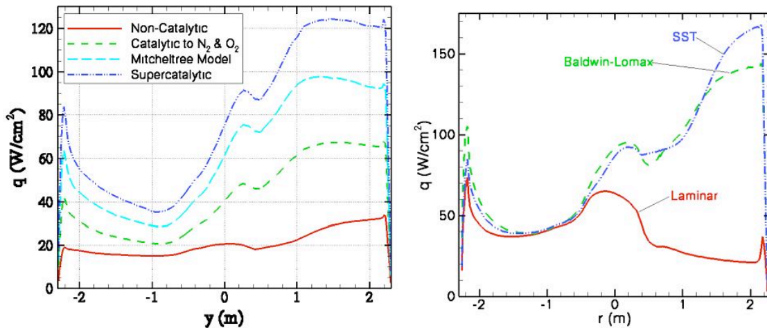
Figure 1. Uncertainties in modeling catalytic heating (left) and turbulent heating (right) 5
