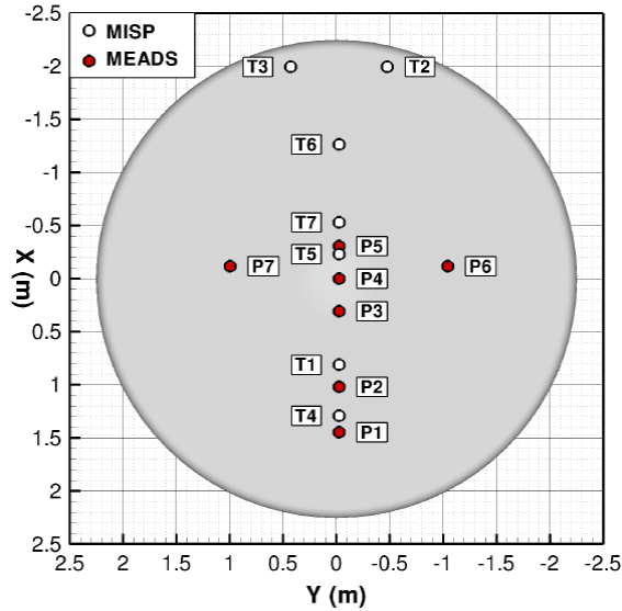
Figure 2. MEDLI sensor locations 3
